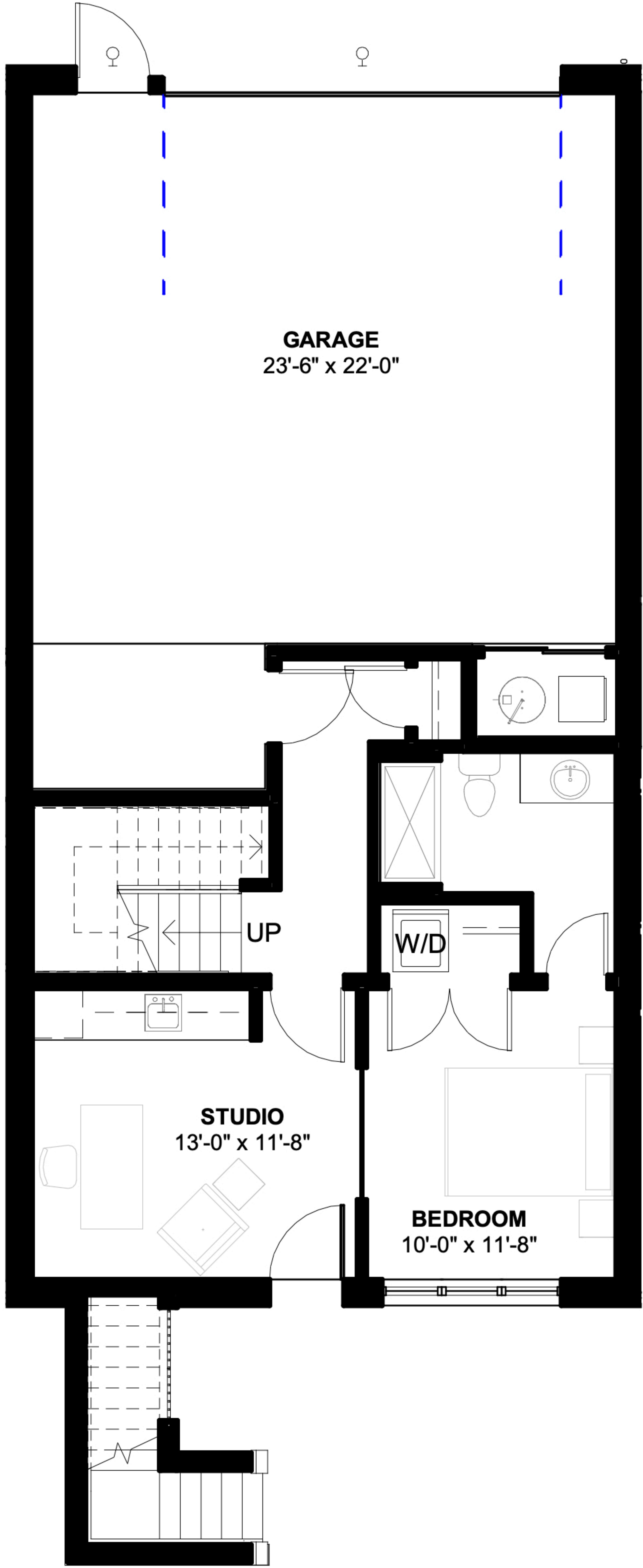
GROUND FLOOR
